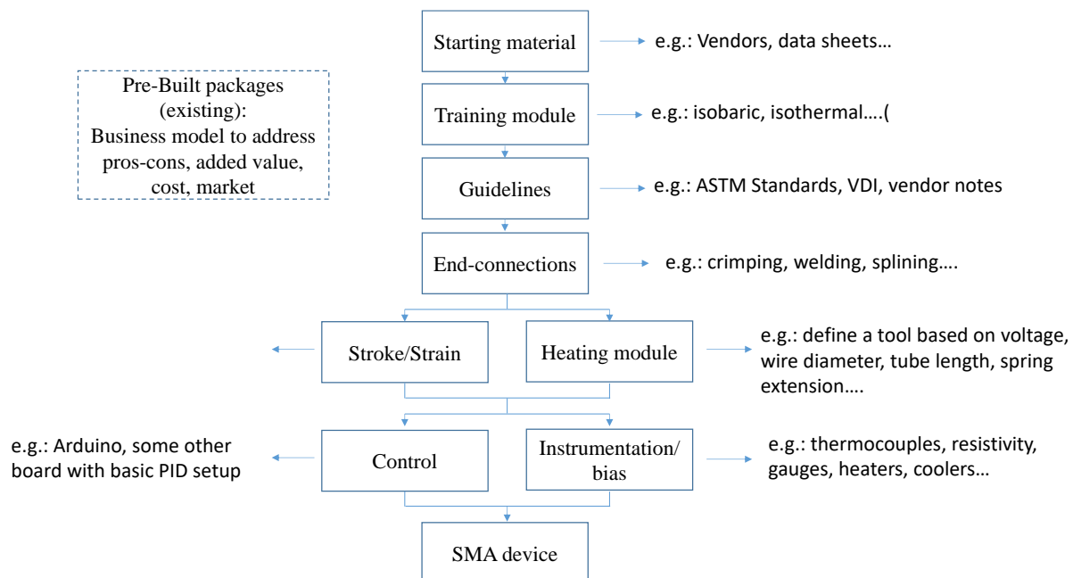
Figure A1: A flow chart showing an example of several modules required for designing an SMA actuator/device. (Not inclusive or generalized).
